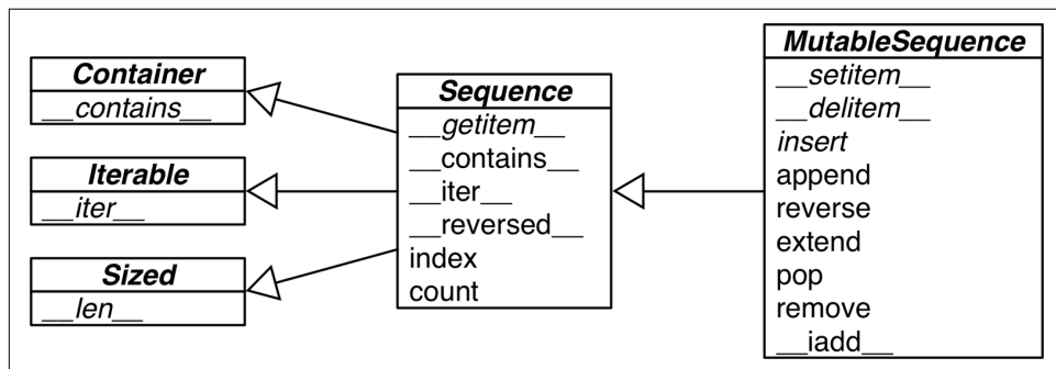
Figure 2-1. UML class diagram for some classes from collections.abc (superclasses are on the left; inheritance arrows point from subclasses to superclasses; names in italics are abstract classes and abstract methods)
