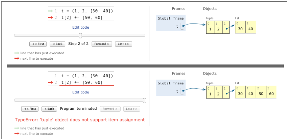
Figure 2-3. Initial and final state of the tuple assignment puzzler (diagram generated by Online Python Tutor)
