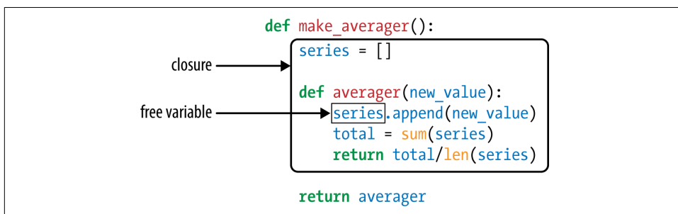
Figure 7-1. The closure for averager extends the scope of that function to include the binding for the free variable series .
