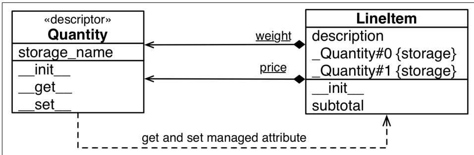
Figure 20-4. UML class diagram for Example 20-2 . Now Quantity has both get and set methods, and LineItem instances have storage attributes with generated names: _Quantity#0 and _Quantity#1 .
