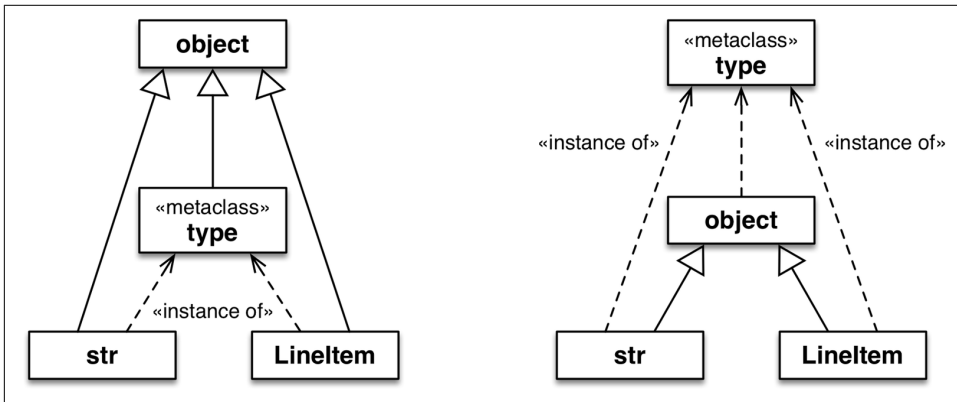
Figure 21-2. Both diagrams are true. The left one emphasizes that str , type , and LineItem are subclasses of object . The right one makes it clear that str , object , and LineItem are instances of type , because they are all classes.
