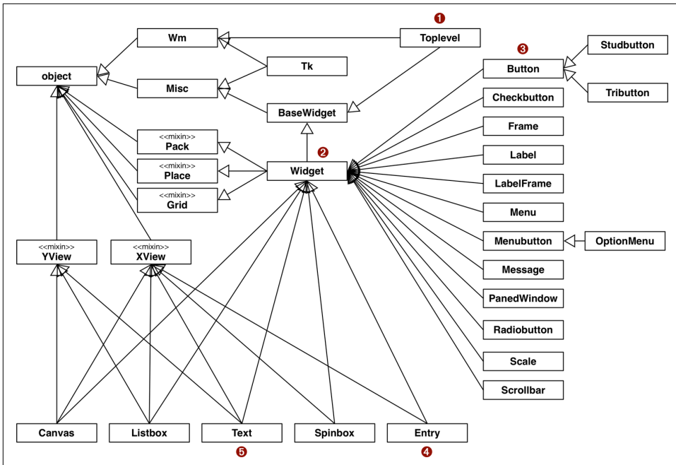
Figure 12-3. Summary UML diagram for the Tkinter GUI class hierarchy; classes tagged «mixins» are designed to provide concrete methods to other classes via multiple inheritance
