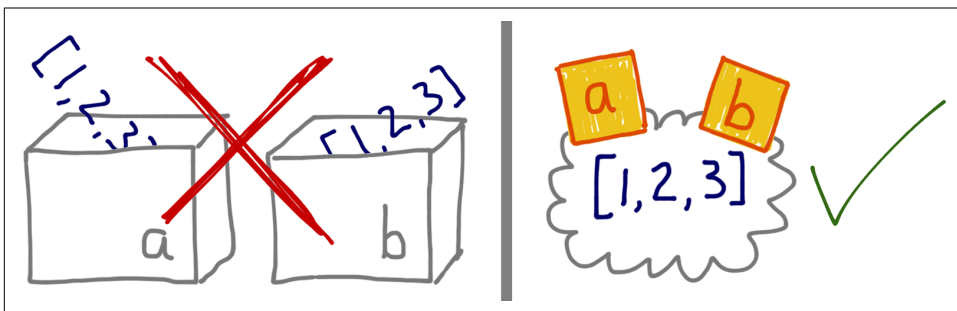
Figure 8-1. If you imagine variables are like boxes, you can't make sense of assignment in Python; instead, think of variables as sticky notes— Example 8-1 then becomes easy to explain
