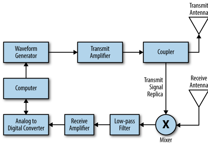
Figure 4-9. The block diagram of a simple FMCW radar system
