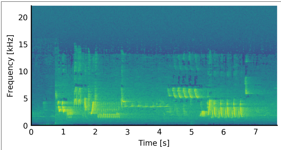
Figure 4-3. Birdsong spectrogram
