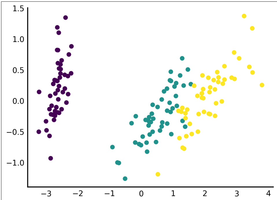
Figure A-3. Principal components of iris dataset computed with normal PCA
