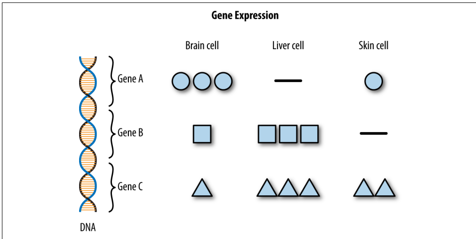
Figure 1-3. Gene expression
