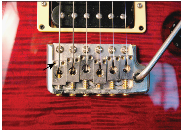
FIGURE 19-1: Turn the saddles' hex screws to raise or lower the action.
